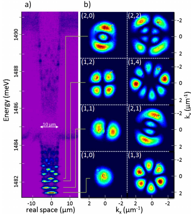
FIG. 1. (Color online) (a) Real space spectrum of a 9 \mu\text{m} mesa at 2 meV negative detuning; upper and lower polariton branches of the 2D and 0D polaritons are clearly visible. (b) K -space images of resonantly excited states from the 0D lower polariton branch. The states can be labeled with two quantum numbers (n, m) . 2|m| gives the number of nodes along \phi on a full circle, while n corresponds to the number of lobes in radial direction.
