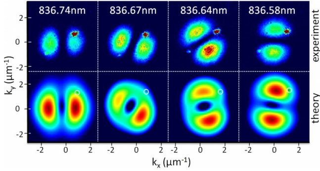
FIG. 3. (Color online) Manipulation of the wave functions of the split first doublet in a 3 \mu\text{m} mesa ( \approx 3 meV negative detuning) by changing the excitation energy while keeping the excitation point constant. Upper part: experiment; lower part: theoretical results. The polariton lifetime in our sample is about 15 ps, which leads to an energy linewidth of the eigenstates much broader than the spectral width of the laser. The lobes rotate due to the different contributions of the eigenstates to the linear response.
