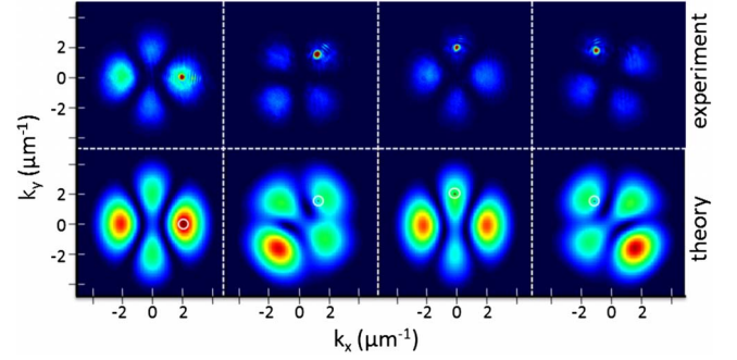
FIG. 2. (Color online) Lobes of the degenerate second doublet state in a 3 \mu\text{m} mesa following the rotation of the laser in k space. The mesa was at zero detuning. The upper part shows the experimental results and the theoretical results from the simulation are shown in the lower part of the figure. The high intensity spot which is visible in each experimental image of this figure is an emission maximum arising from the laser light transmitted directly through the cavity beside the mesa. This makes it easy to observe the excitation angle. In the simulation images the laser position is marked by a circle.
